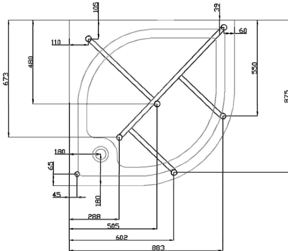
Fig 1 Legs and frame position (top view)
